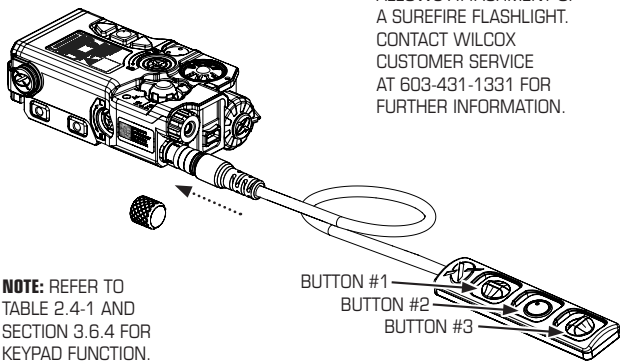
Figure 3.3-1 Attaching/Detaching the Three Button Pressure Pad to/from the RAID Xe
