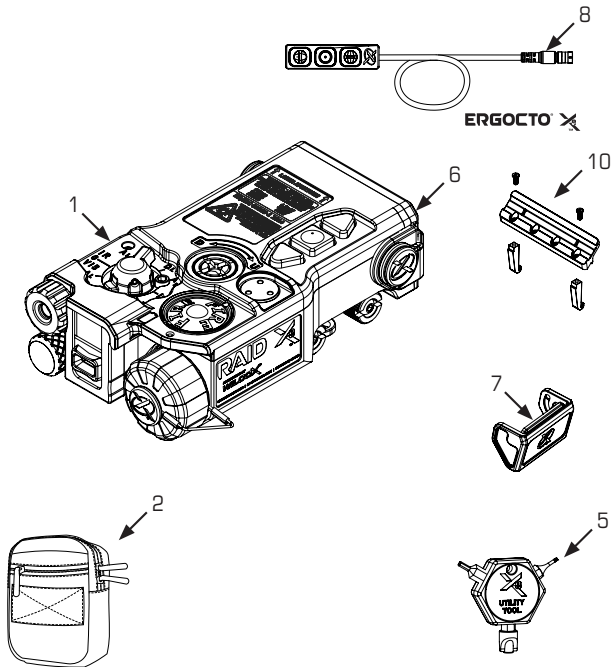
Figure 2.2-1 Major Component Identification
