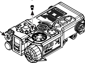
Figure 3.2-1 Installing the High Power Lockout Screw on the RAID Xe
