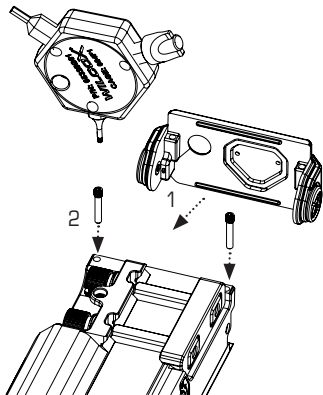
Figure 4.4-1. Attaching the RAID Xe Laser Safety Hood
