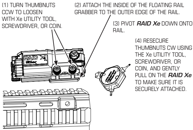
Figure 3.1-1 Mounting the RAID Xe to the MIL-STD-1913 Rail (12 O'Clock Mounting Depicted)
