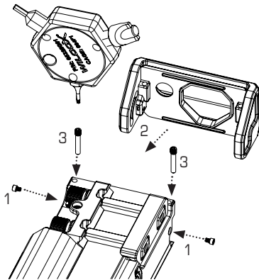
Figure 4.4-2. Attaching the RAID Xe Laser Safety Visor
