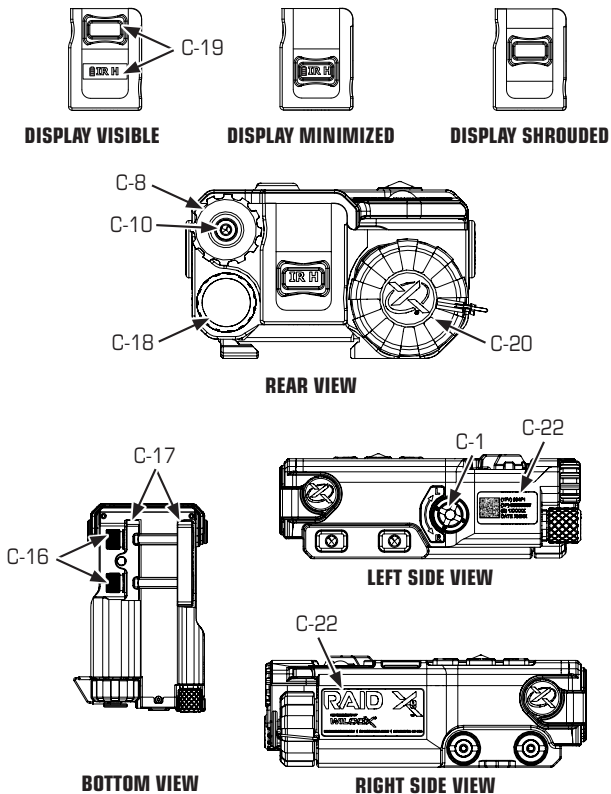
Figure 2.3-2 Subcomponent Identification - RAID Xe (2 of 2)
